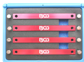
MB7 Afstelset / Kit de calage Mercedes M276, M157, M278, C 216, 217, 218, C/A 207, C/X 218, R 172, 231, V 222, W 166, W 205, W 212, 463, W/S 212, W/S/C 204, W/V 221, 222, 251, X 166, 204
